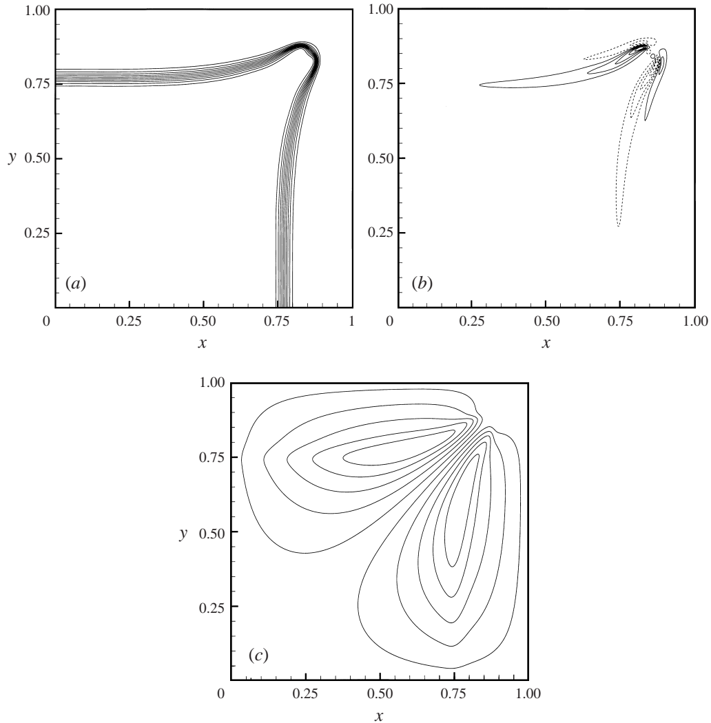
FIGURE 7. Contours of concentration (a), vorticity (b, negative values dashed), and perturbation streamfunction (c) for Pe = 800 , \alpha = 2.0 , \mu_m = 3.0 , c_m = 0.37 at t = 0.40 . All plots are scaled with the instantaneous maxima.
